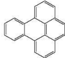
benzo[e]pyrene
