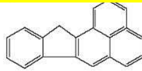
benzo[b]fluoranthene
